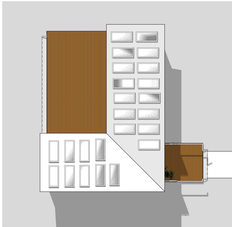
② ROOF PLAN 1/8" = 1'-0"
