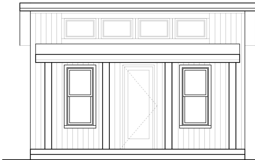
③ South Elevation 3/16" = 1'-0"
