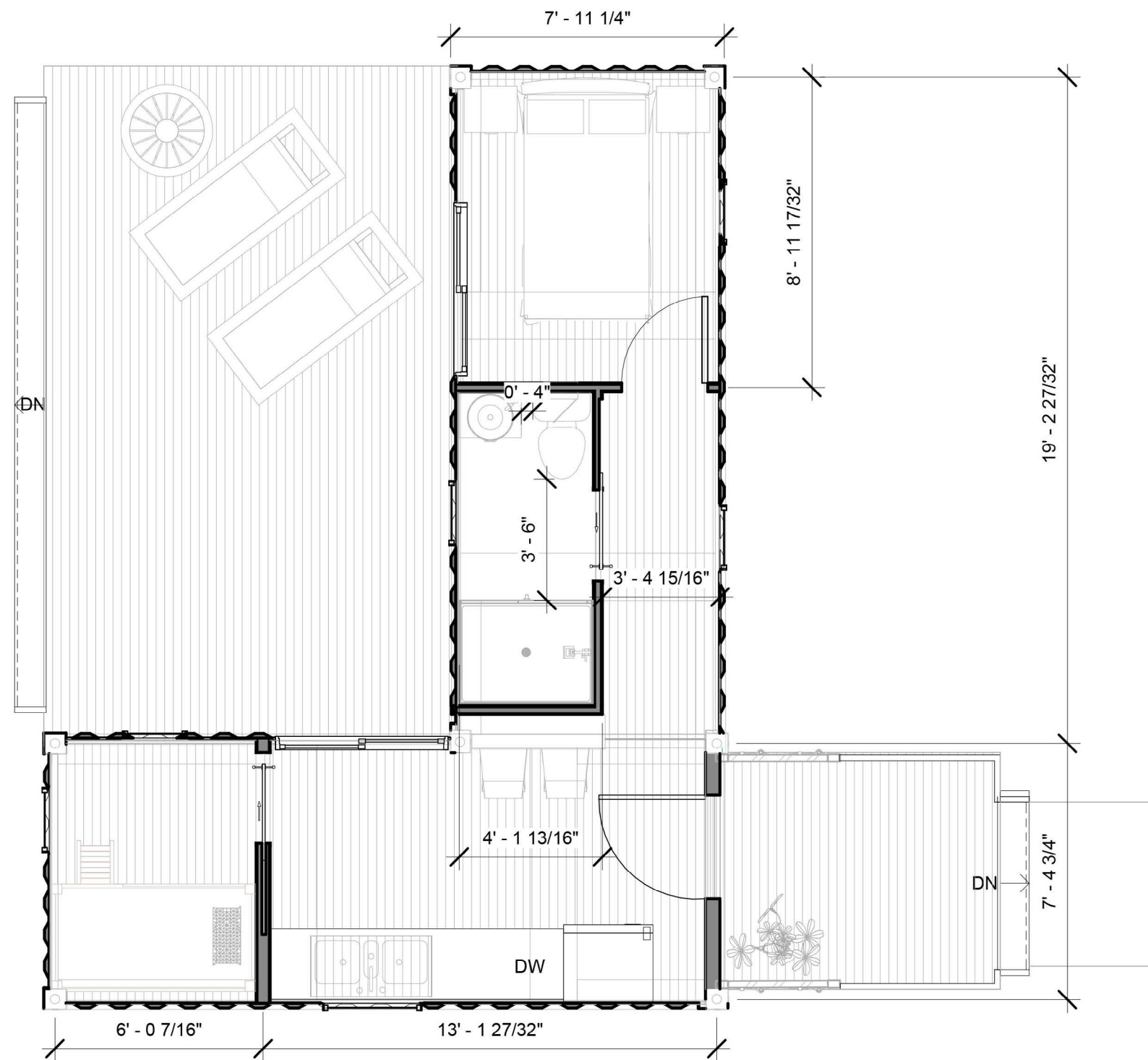
① Floor Plan 1/4" = 1'-0"
