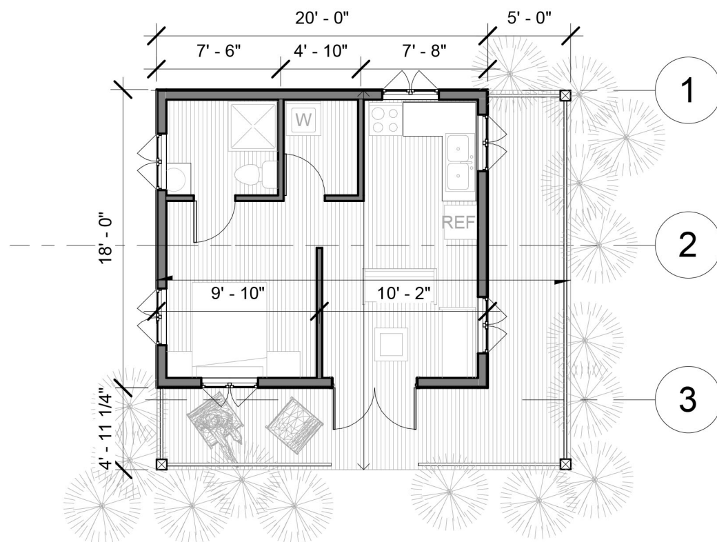
① First Floor 1/8" = 1'-0"
