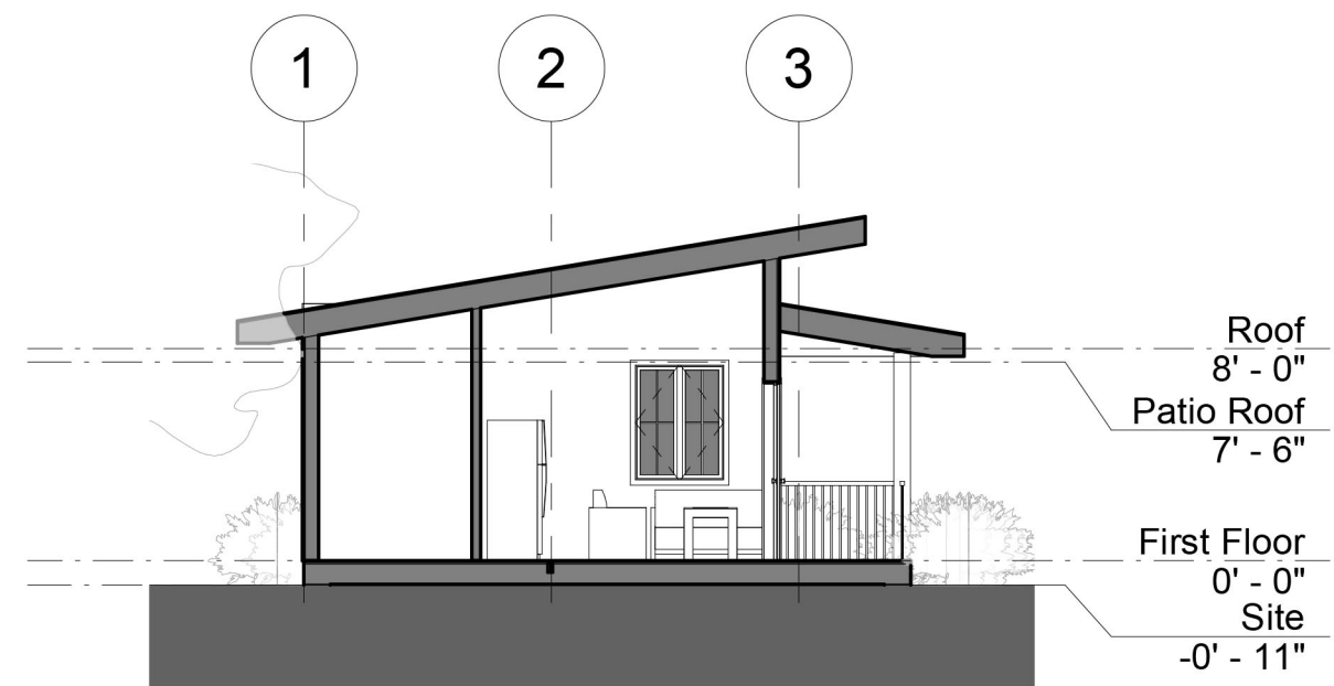
④ Section 1 1/8" = 1'-0"
