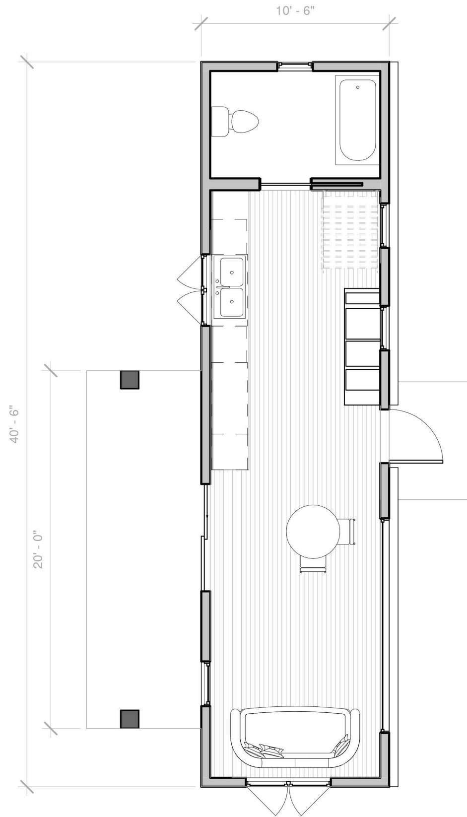
① First Floor Plan 3/16" = 1'-0"
