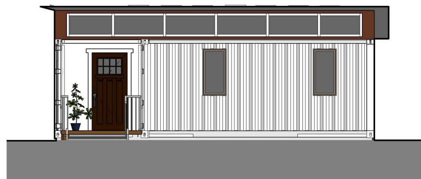
⑤ FRONT VIEW 1/8" = 1'-0"
