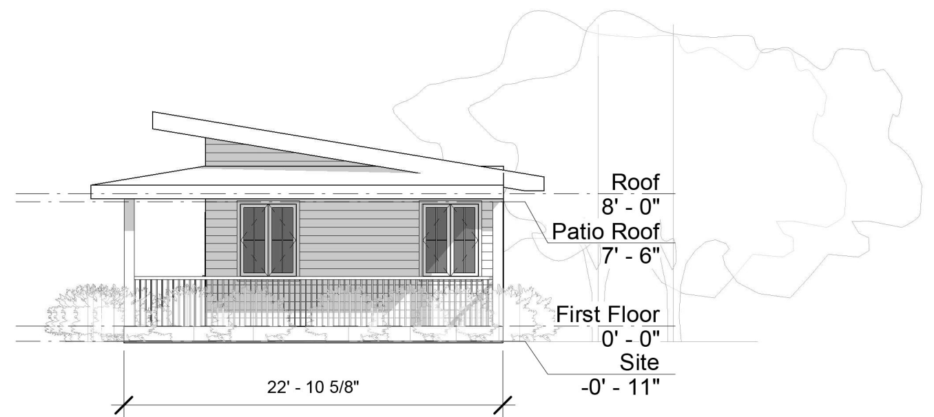
③ East 1/8" = 1'-0"
