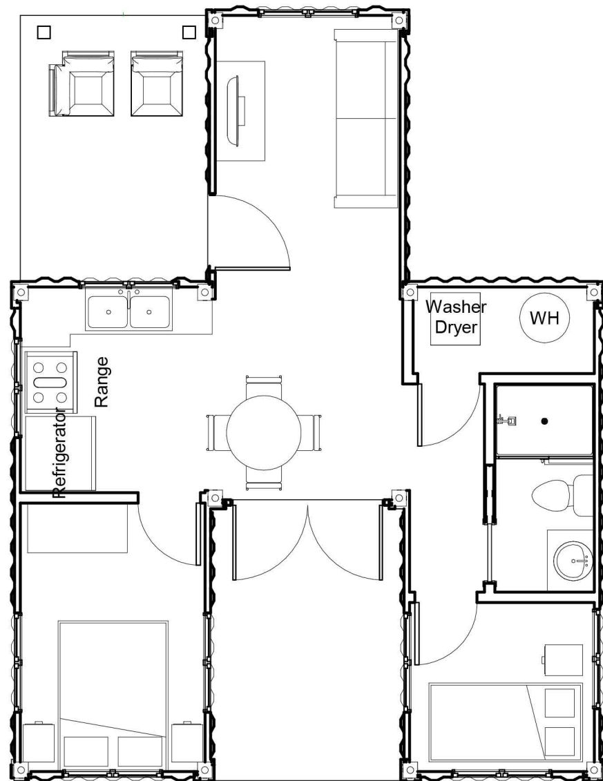
FLOOR PLAN 3/16" = 1'-0"
